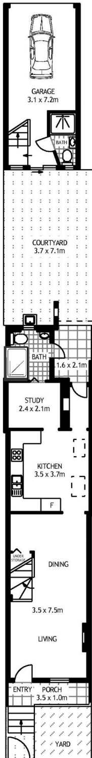
GROUND FLOOR
