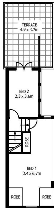
FIRST FLOOR
