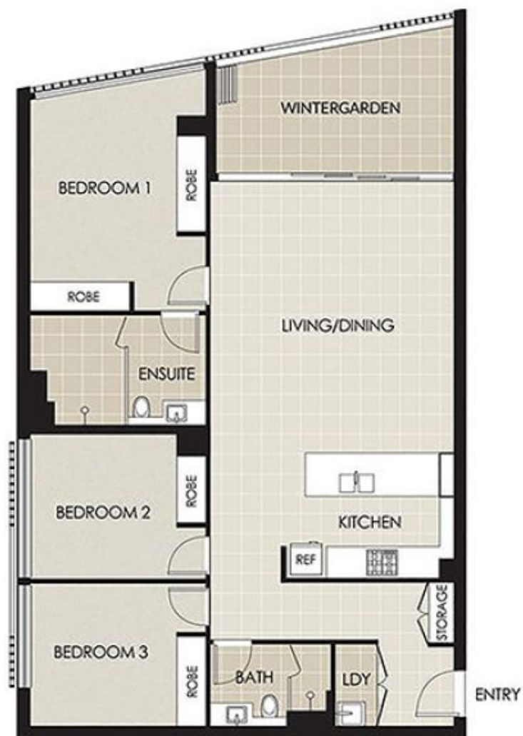
APARTMENT FLOOR PLAN
