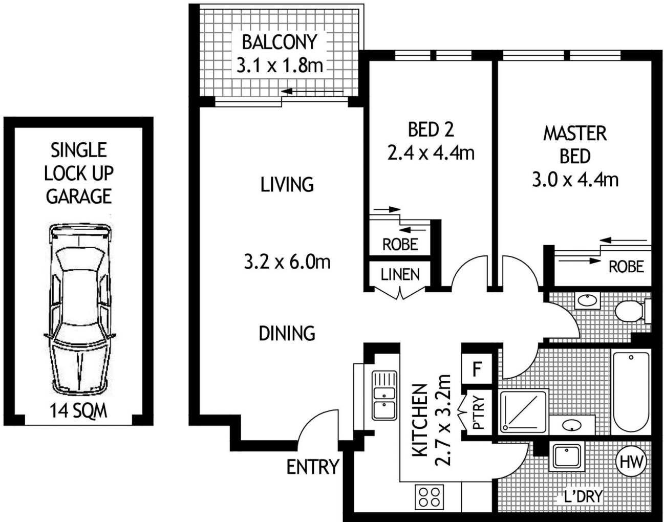
FIRST FLOOR
