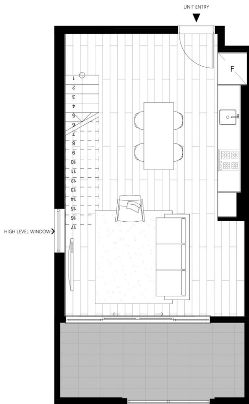
LOWER FLOOR
