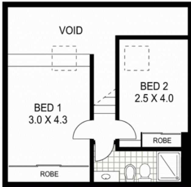
THIRD FLOOR
