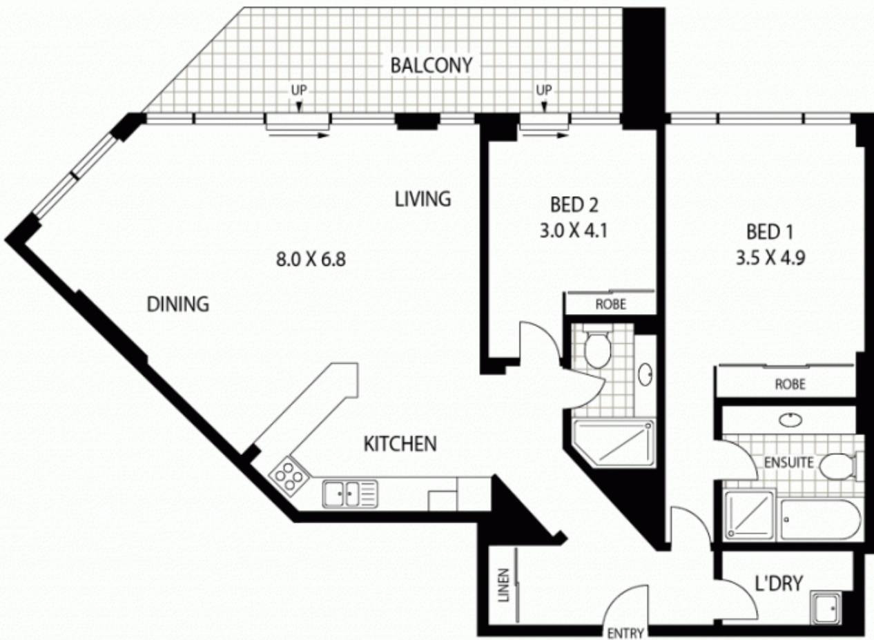
SIXTEENTH FLOOR
