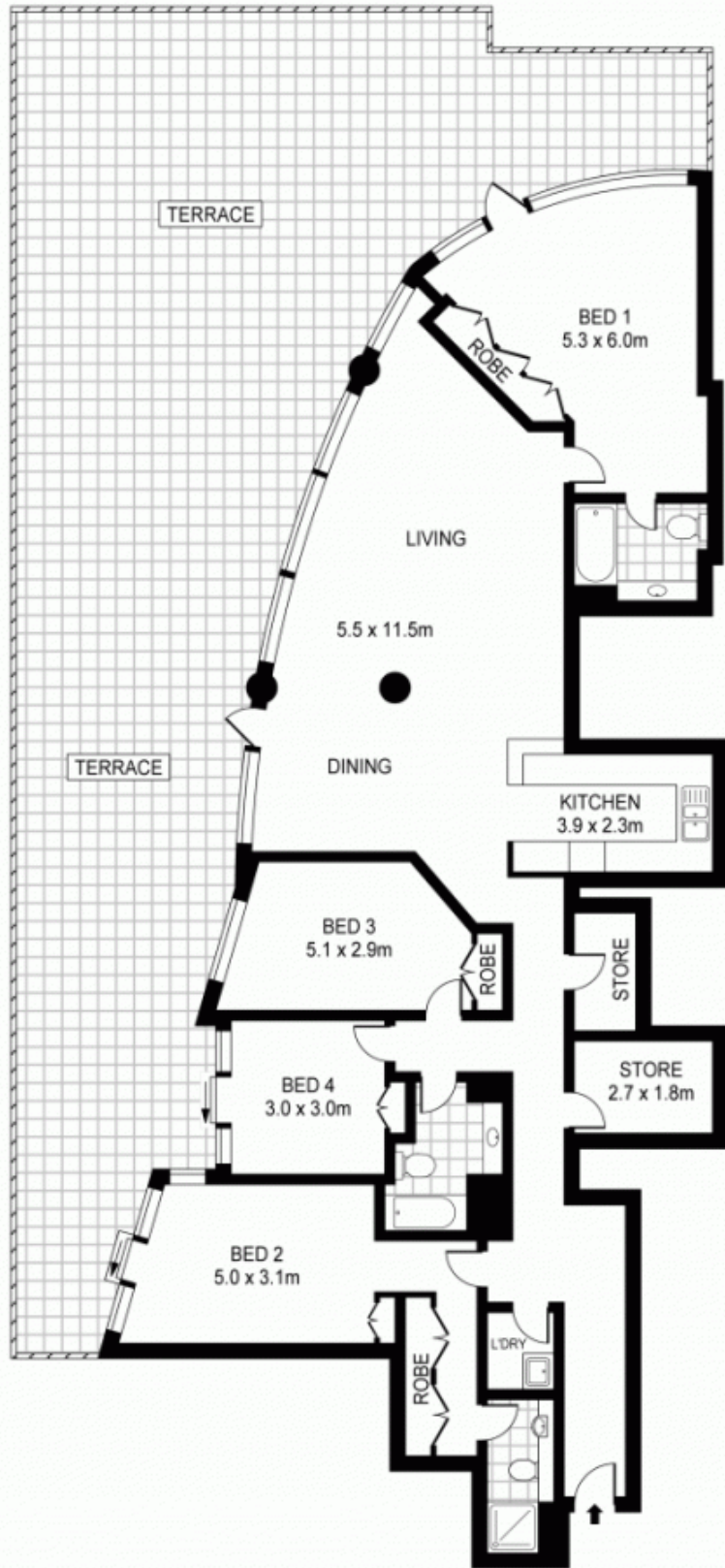
SEVENTEENTH FLOOR
