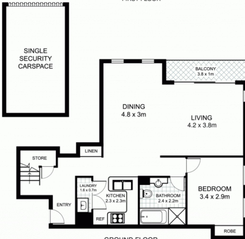
GROUND FLOOR
