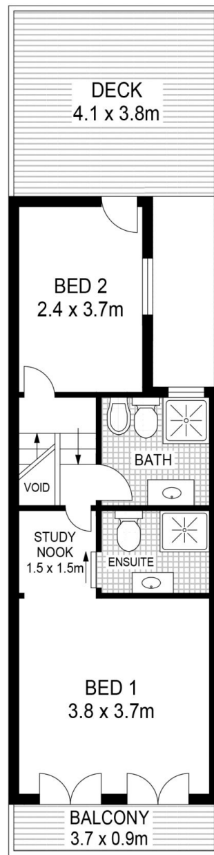
FIRST FLOOR
