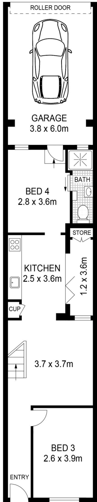
GROUND FLOOR
