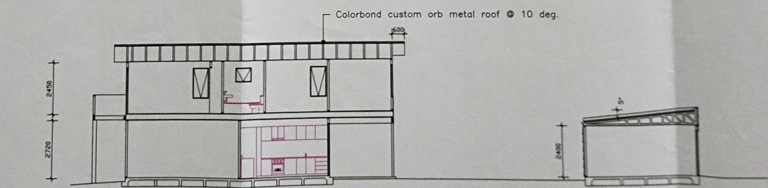
SECTION 1-1
