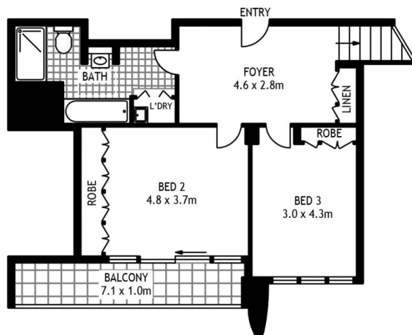
THIRTEENTH FLOOR
